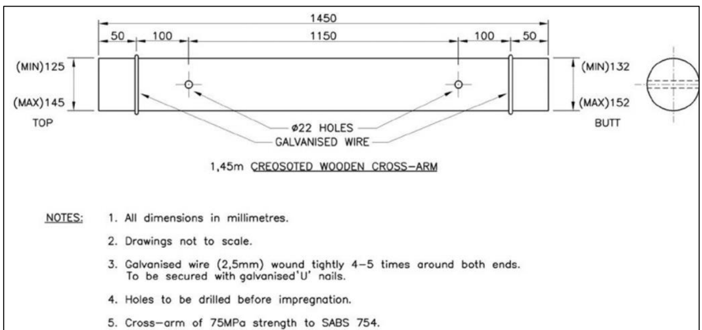
Figure 1 – Hole positions on 1,45 m cross-arms
